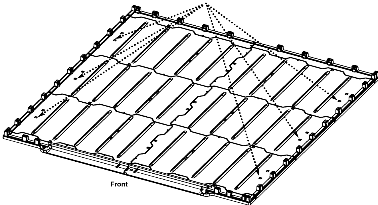
First of two anchor holes in each floor panel
