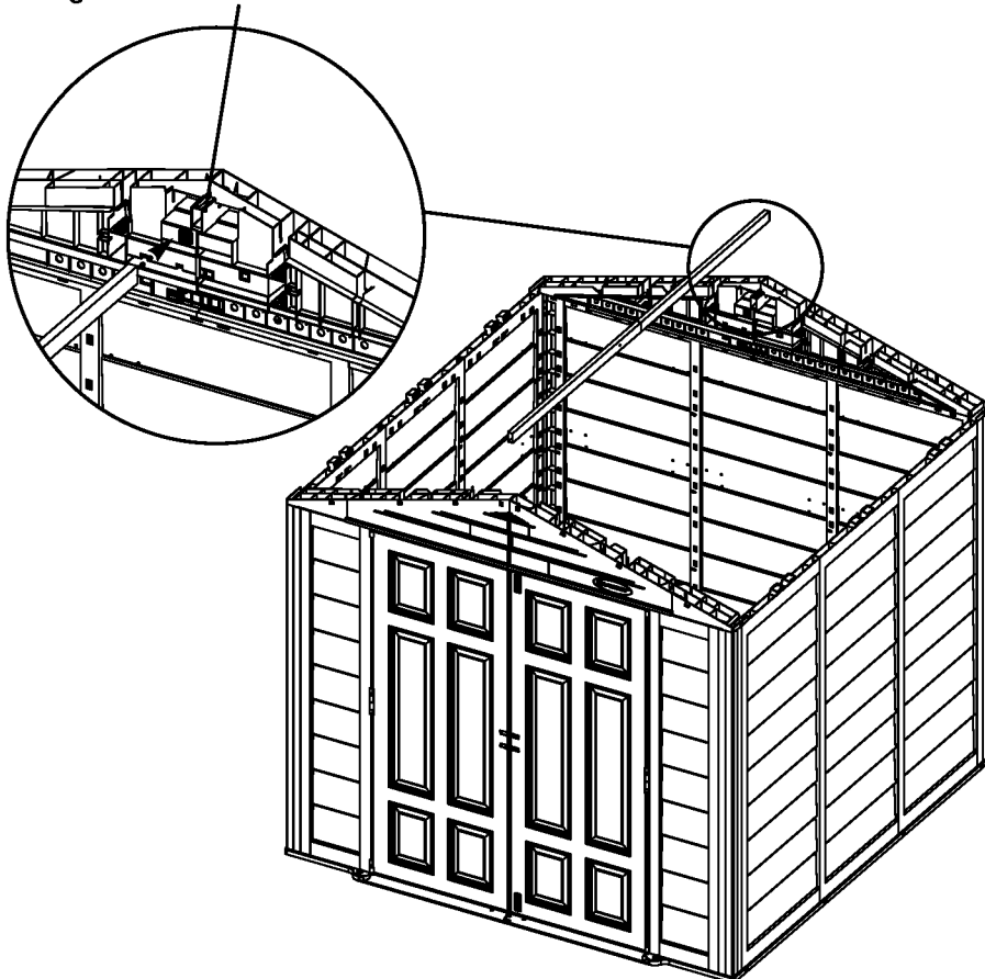
Rectangular boss in center of Front Header
