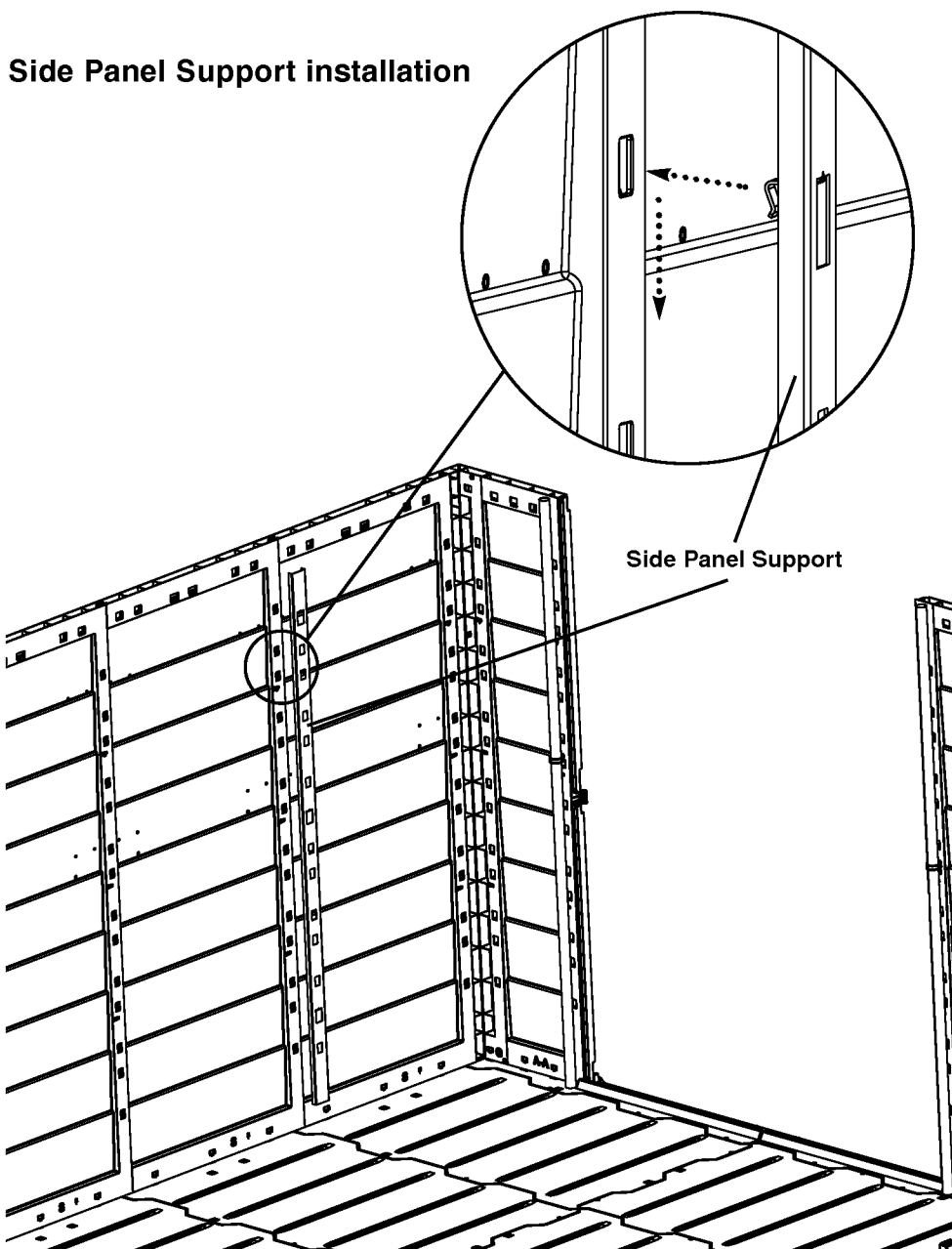
View from inside shed - roof and doors not shown
