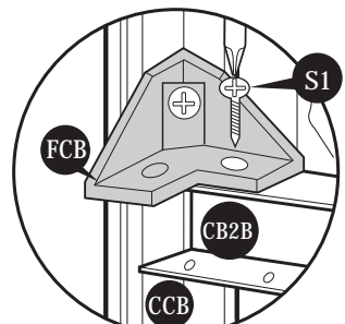
Fig.4: Use (S1) screws. Fix (CB2B) to (FCB).
