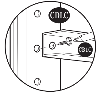
Fig.3: Use (S1) screw. Fix (CB1C) to (CDLC).
