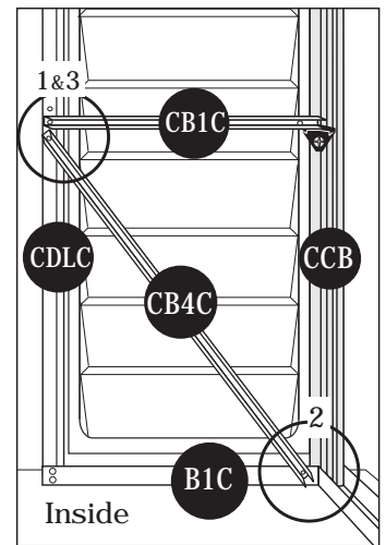
Fig.2: Use (S1) screw. Fix (CB4C) to base (B1C)
