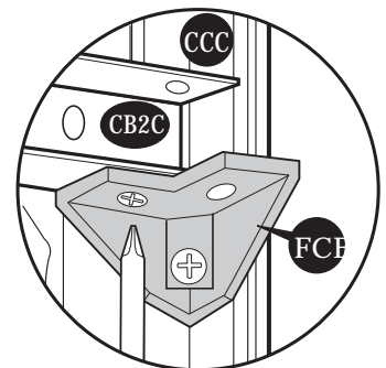
Fig. 4: Use (S1) screw. Fix (CB2C) to (FCB).
