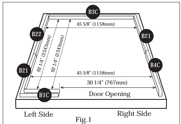
Plywood Floor
