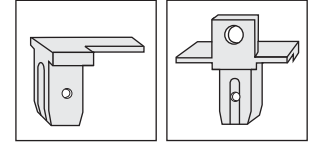
DOOR COLUMN FITTING (FDCLC) MIDDLE COLUMN FITTING (FMC)
