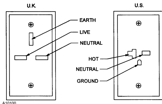
Figure 1A. 230V Outlets
