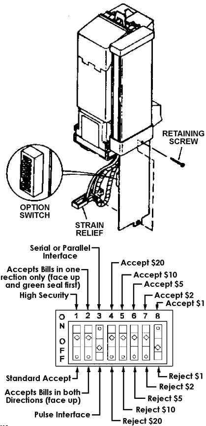
Figure 11. Validator Switch Module
