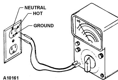
Figure 1B. Testing 115V Outlet
